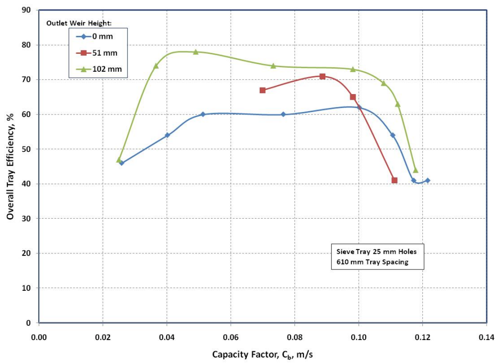
Figure 7. Effect of Weir Height on Efficiency for 14% Hole Area Tray ( C_6/C_7 at 0.276 bar Pressure)
